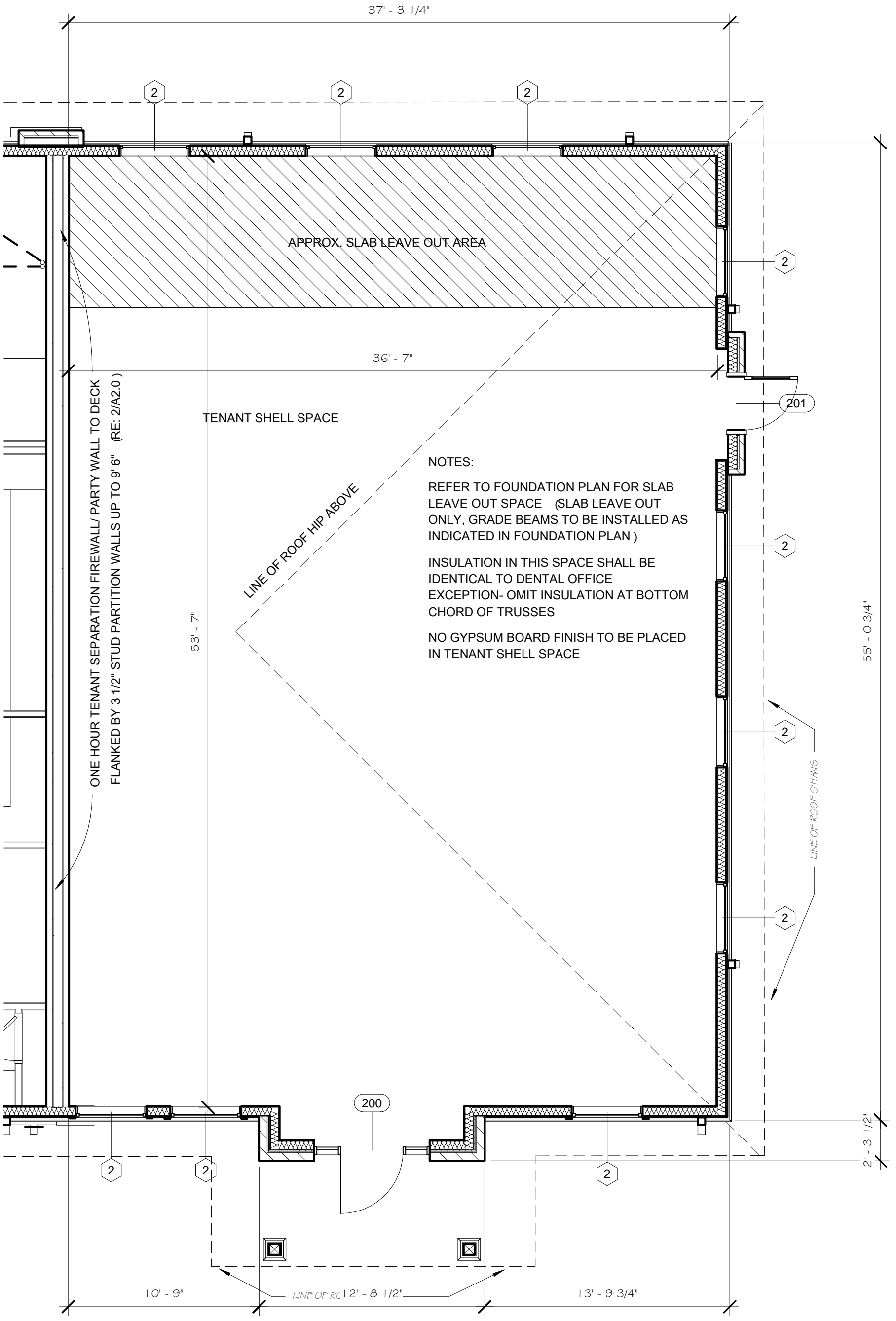
① Lease Building Shell w dimensions 3/16" = 1'-0"
