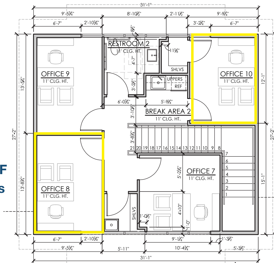
2 SECOND FLOOR PLAN SCALE: 3/16" 1'-0"
